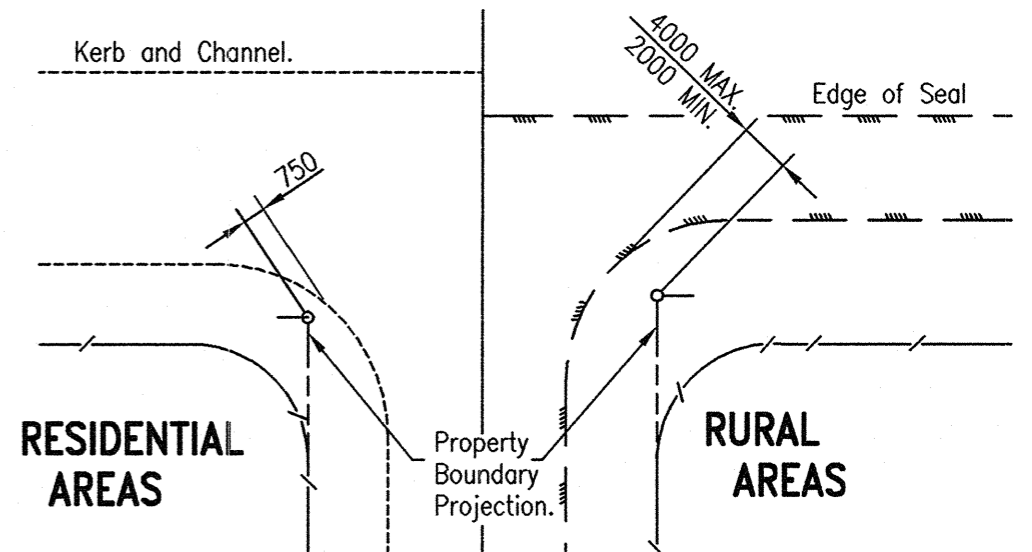
TYPICAL STREET SIGN LOCATIONS N.T.S.
