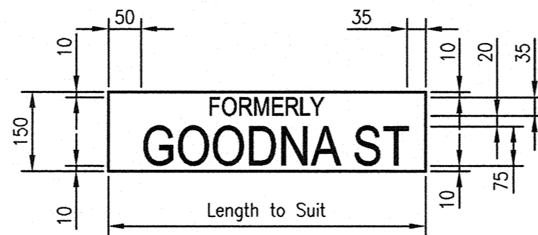
SUPPLEMENTARY SIGN PLATE DETAIL N.T.S.
