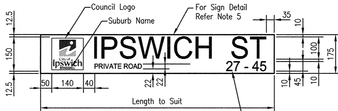
PRIVATE ROADS SIGN PLATE DETAIL N.T.S.
