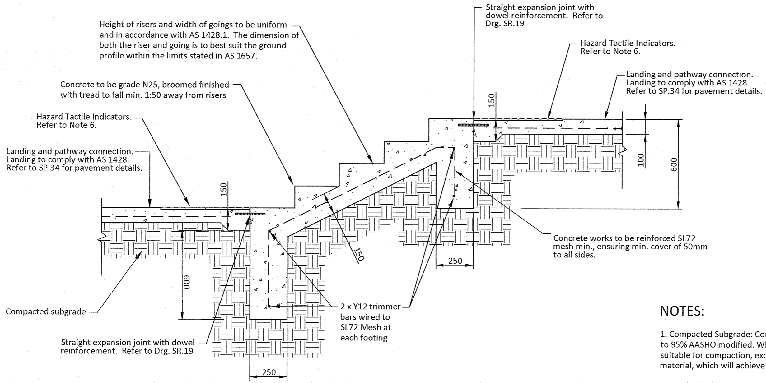
CONCRETE STEPS SECTION
