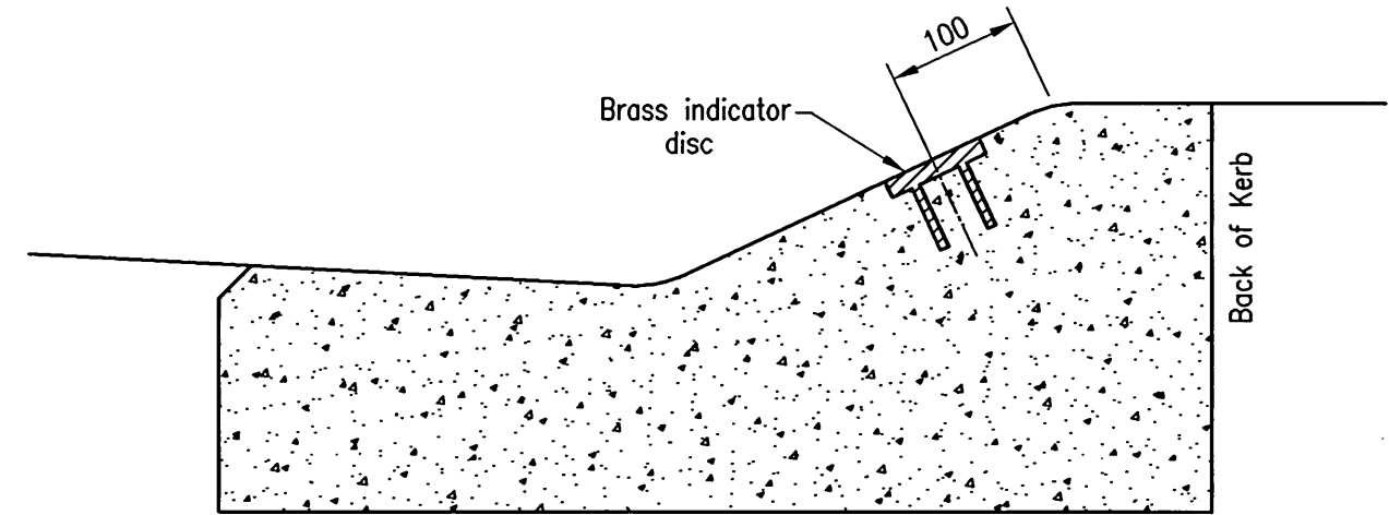
MOUNTABLE KERB AND CHANNEL
