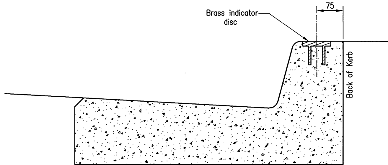
BARRIER KERB/KERB AND CHANNEL
