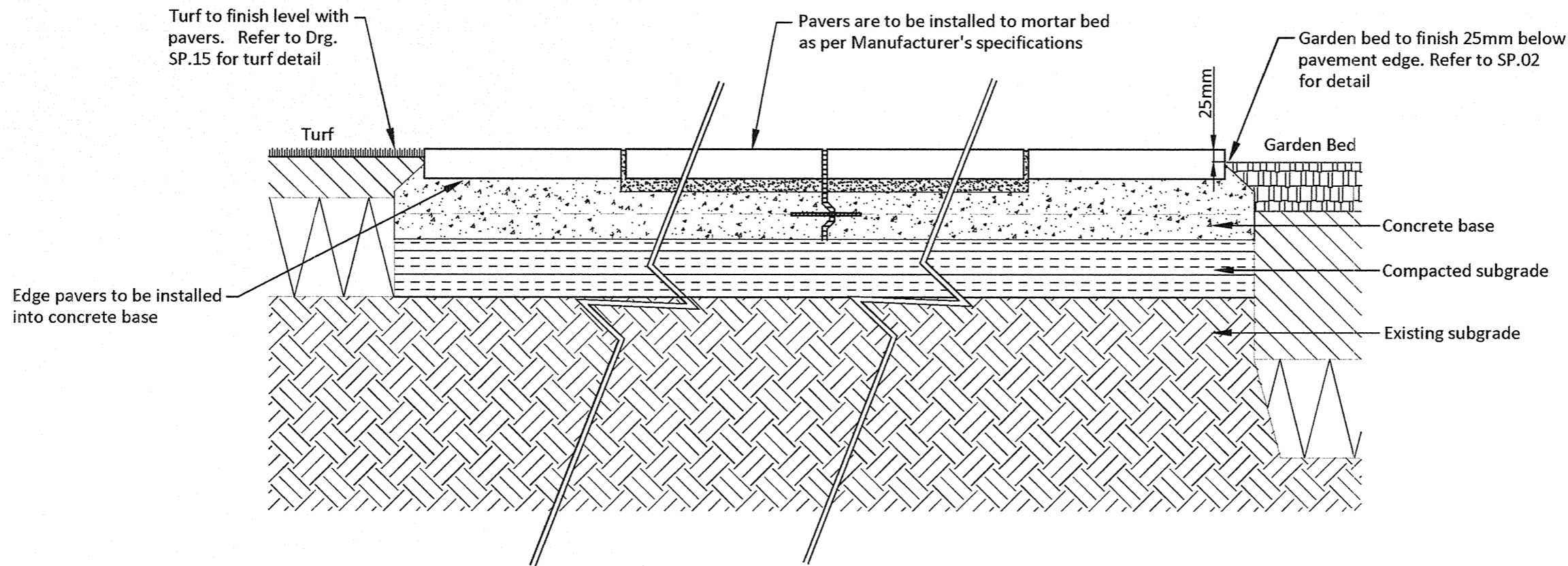
SECTION - TURF TO PAVED FOOTPATH TO GARDEN BED
