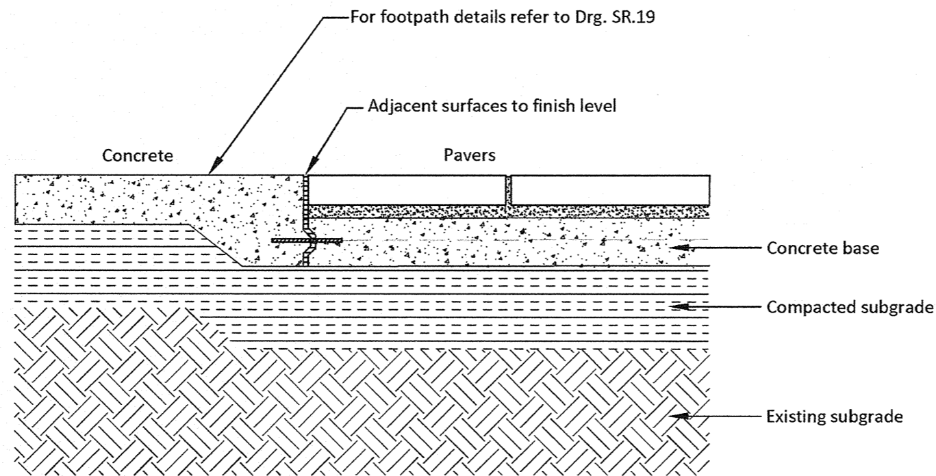
SECTION - CONCRETE TO PAVERS
