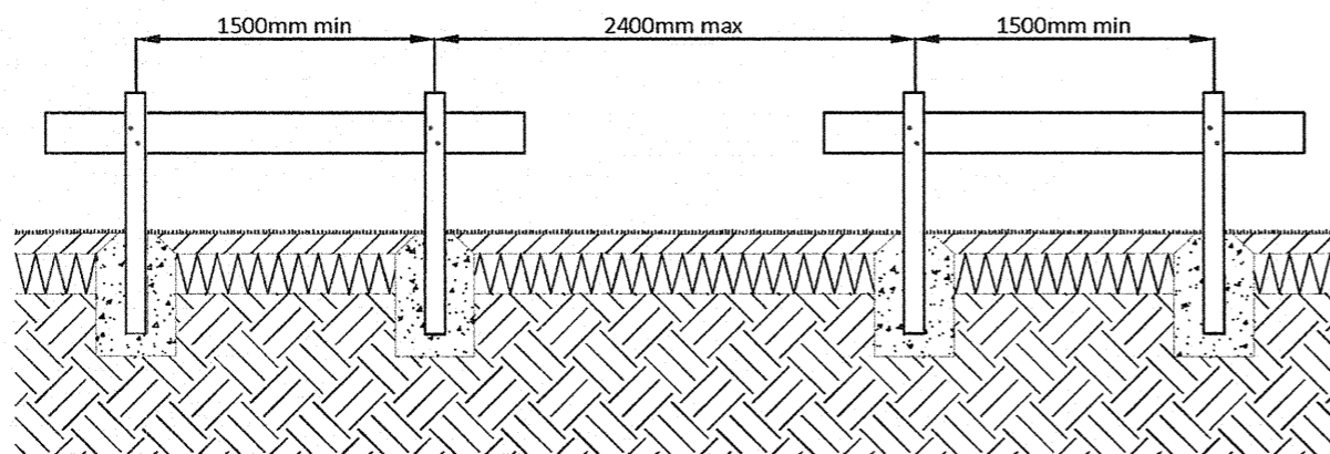
ELEVATION: POST AND RAIL SCALE: 1:40
