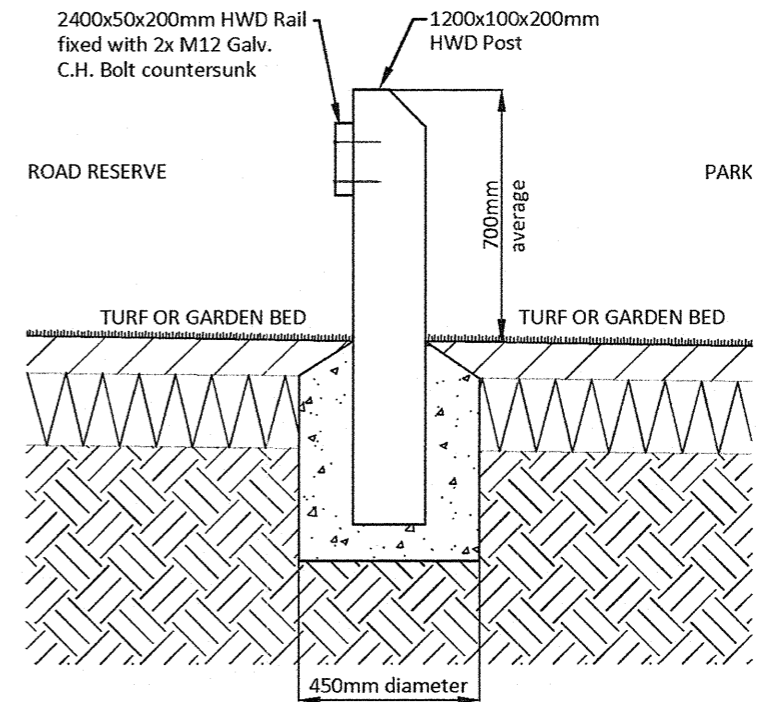
SECTION: POST AND RAIL SCALE: 1:20
