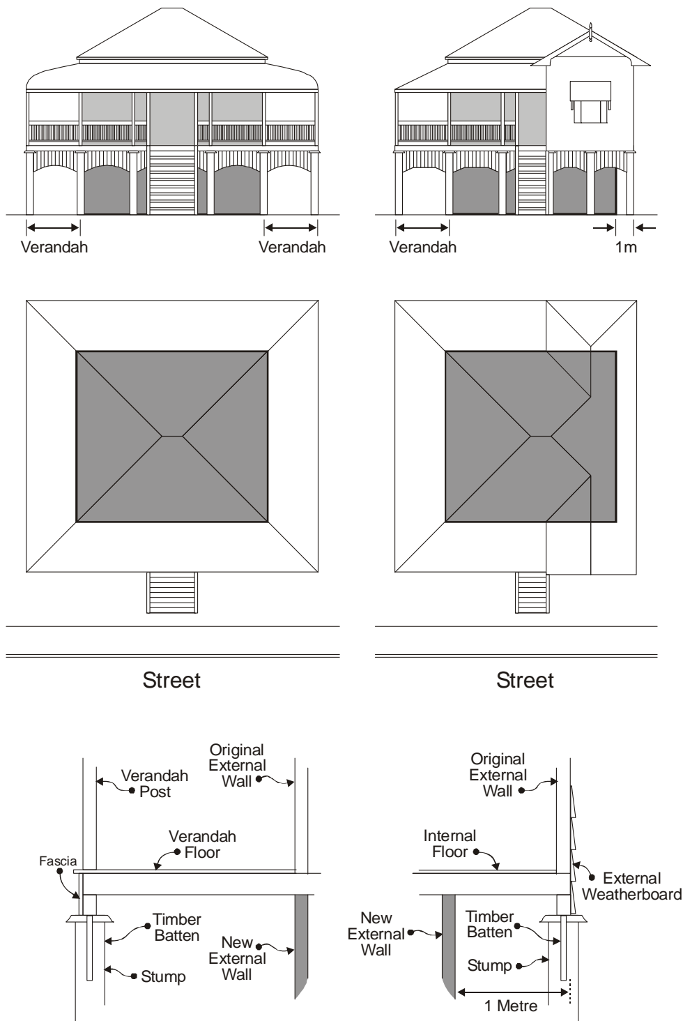
Figure 2: Closing in Underneath a Building
