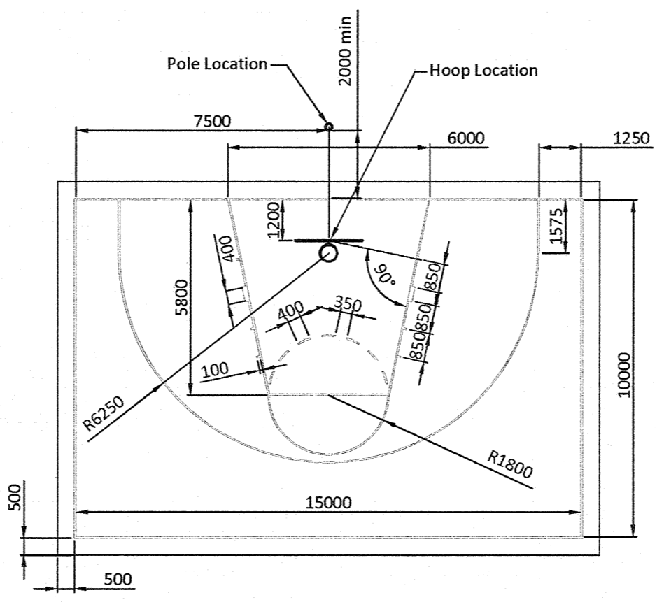
PLAN: LINE MARKING SCALE: 1:150
