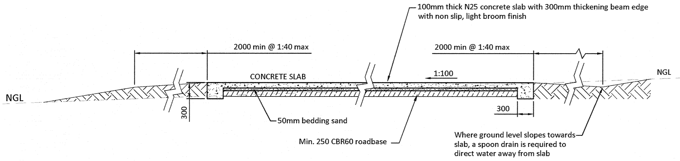
SECTION: TYPICAL SECTION SCALE: 1:40
